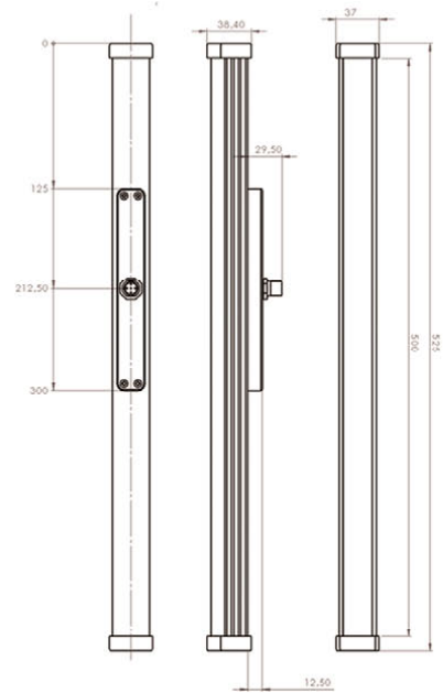
Flex bar light e.g. BLflex-0250
