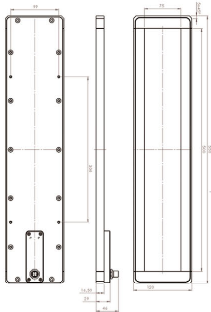
Flex back light e.g. DBLflex-0750
